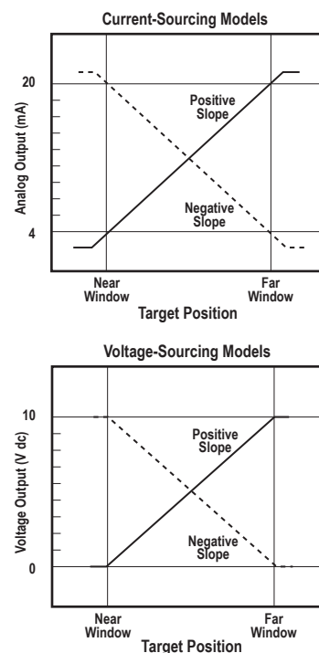
Figure 2. Positive and Negative Output Slopes
