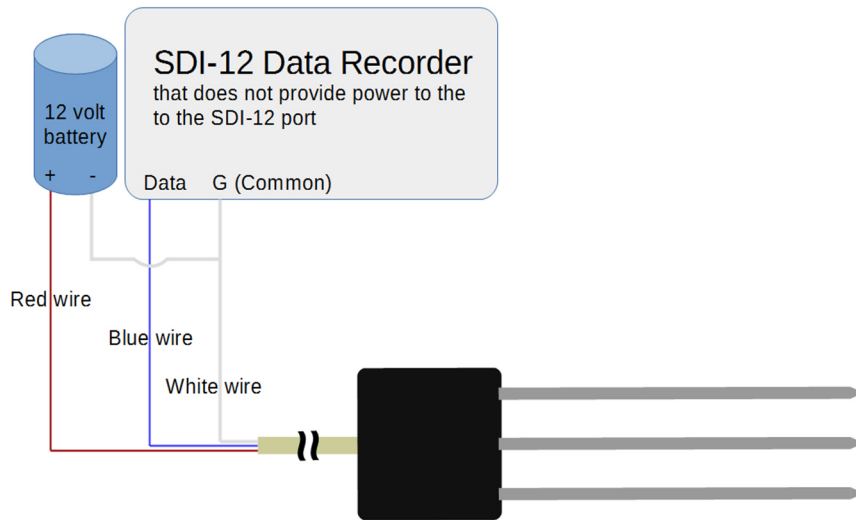
Diagram for the data recorder using an external battery
