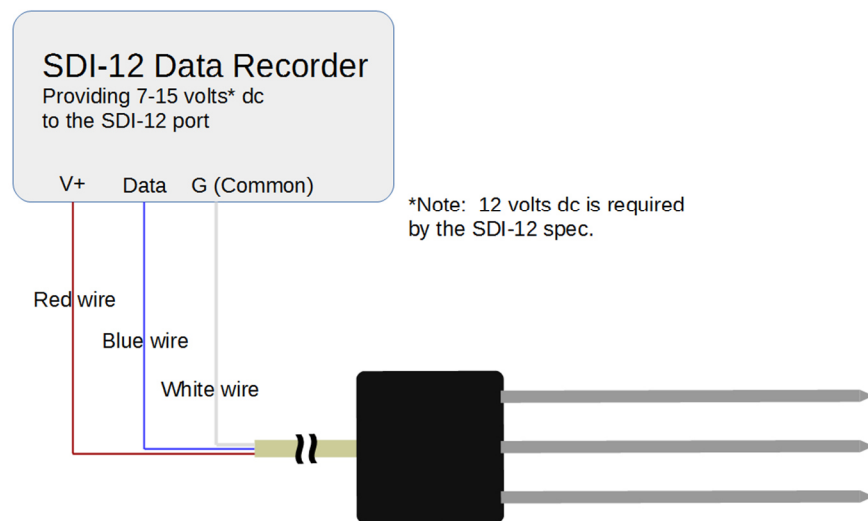
Diagram for a data recorder providing power to the SDI-12 port
